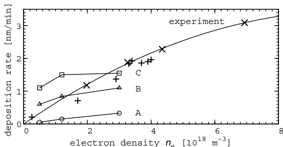
Fig. 6. Deposition rate vs. electron density for a He (x) and an Ar (+) discharge. The results of modeling are included for He: A (circles): atomic data according [4], B (triangles): atomic data multiplied by a factor of 10, C (squares): as B and sticking coefficients according [9].
