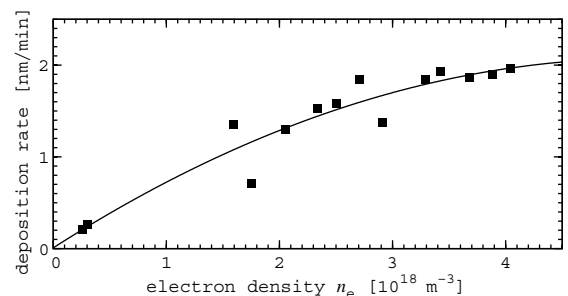
Fig. 2. Deposition rate versus electron density measured for an injection of 0.5 sccm \text{CH}_4 into Ar-plasmas.
