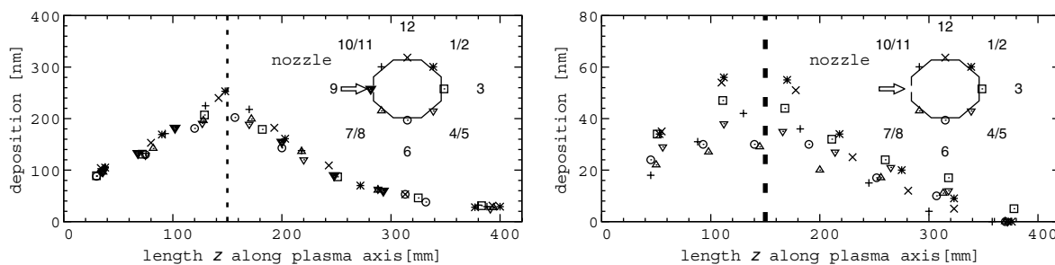
Fig. 3. Deposition pattern on the eight collectors for a H-plasma (left, n_e = 4.0 \times 10^{17} \text{ m}^{-3} ) an Ar-plasma (right, n_e = 2.3 \times 10^{18} \text{ m}^{-3} ).
