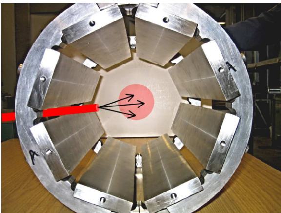
Fig. 1. Eight tiles bearing Si-collectors are arranged around the plasma column. Hydrocarbons are injected from the left hand side.
