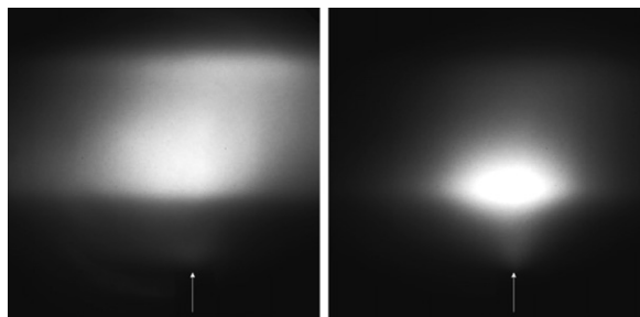
Fig. 4. CH-emission patterns in a He discharge for low (left, n_e = 5 \times 10^{17} \text{ m}^{-3} ) and high (right, n_e = 3 \times 10^{18} \text{ m}^{-3} ) electron density. The position of the nozzle is indicated by the arrow.
