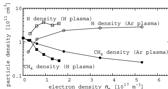
Fig. 5. Particle density of H and \text{CH}_4 vs. n_e for methane injection into hydrogen (squares) and argon (circles) plasmas.
